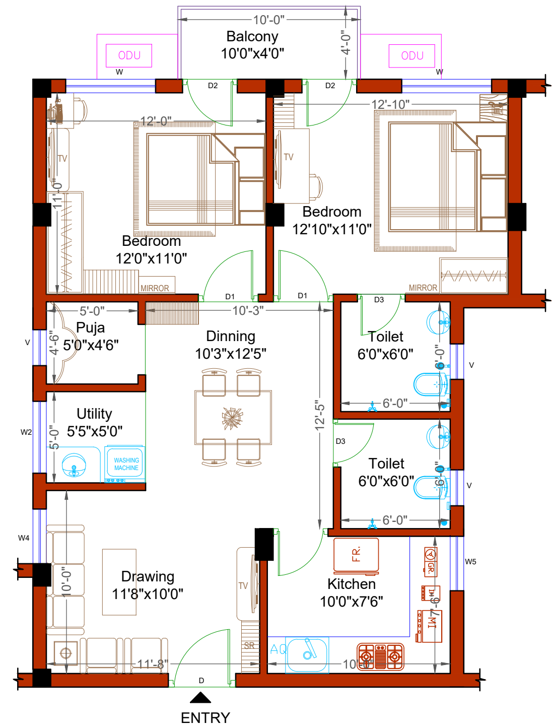
TYPICAL FLAT NO -102 TO 502
