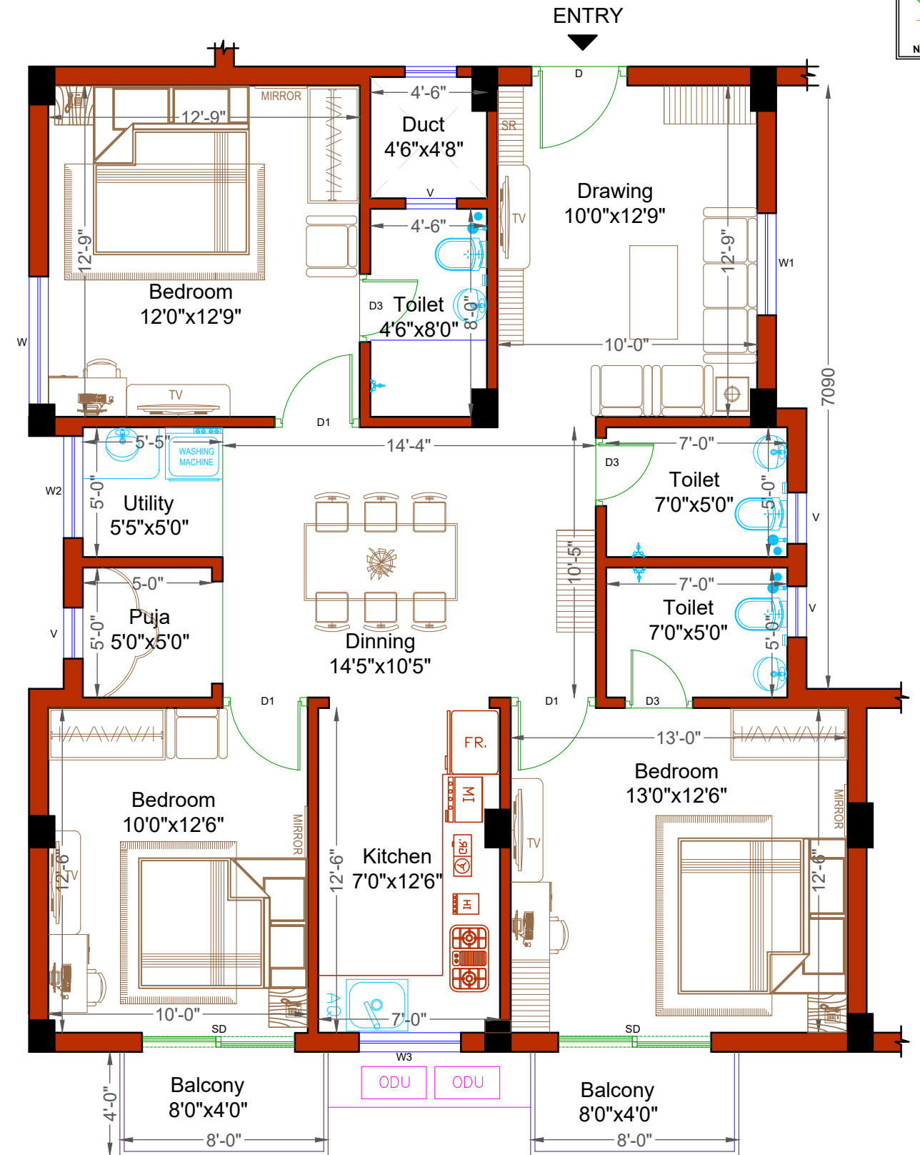
TYPICAL FLAT NO -107 TO 507
